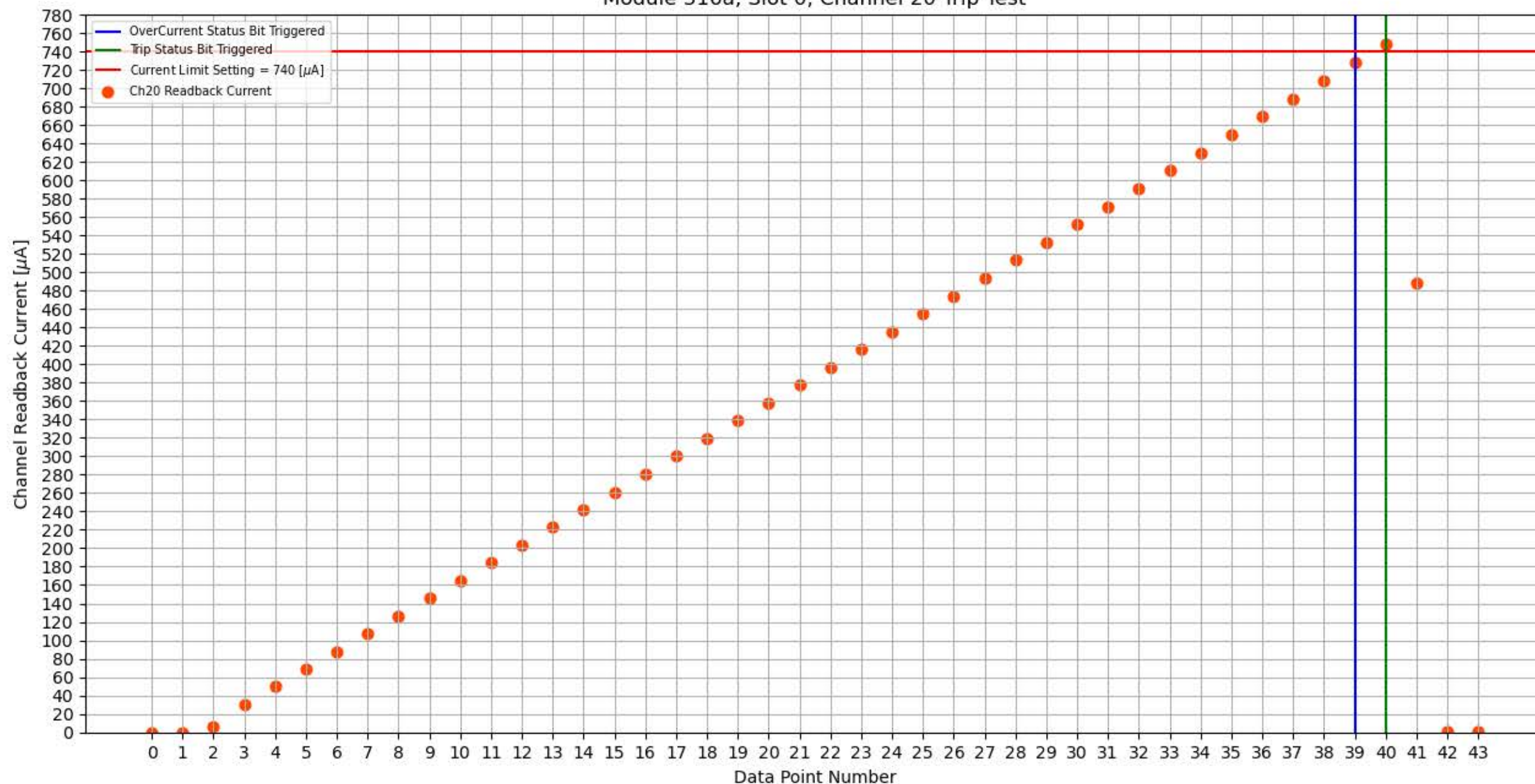
Module 316a, Slot 0, Channel 20 Trip Test
