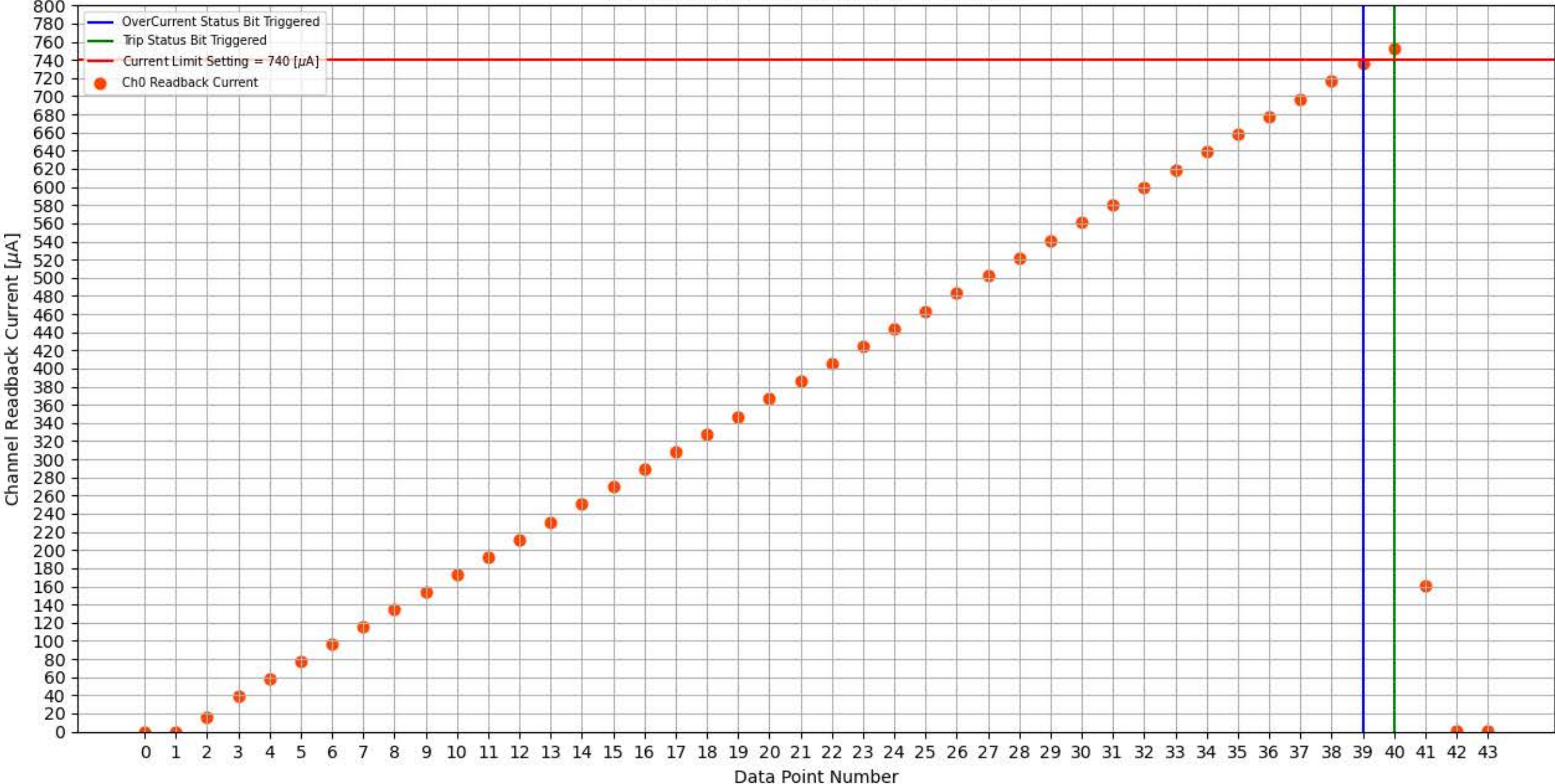
Module 316a, Slot 0, Channel 0 Trip Test
