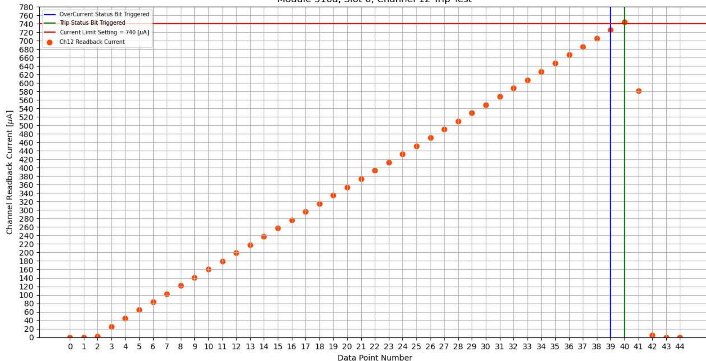
Module 316a, Slot 0, Channel 12 Trip Test
