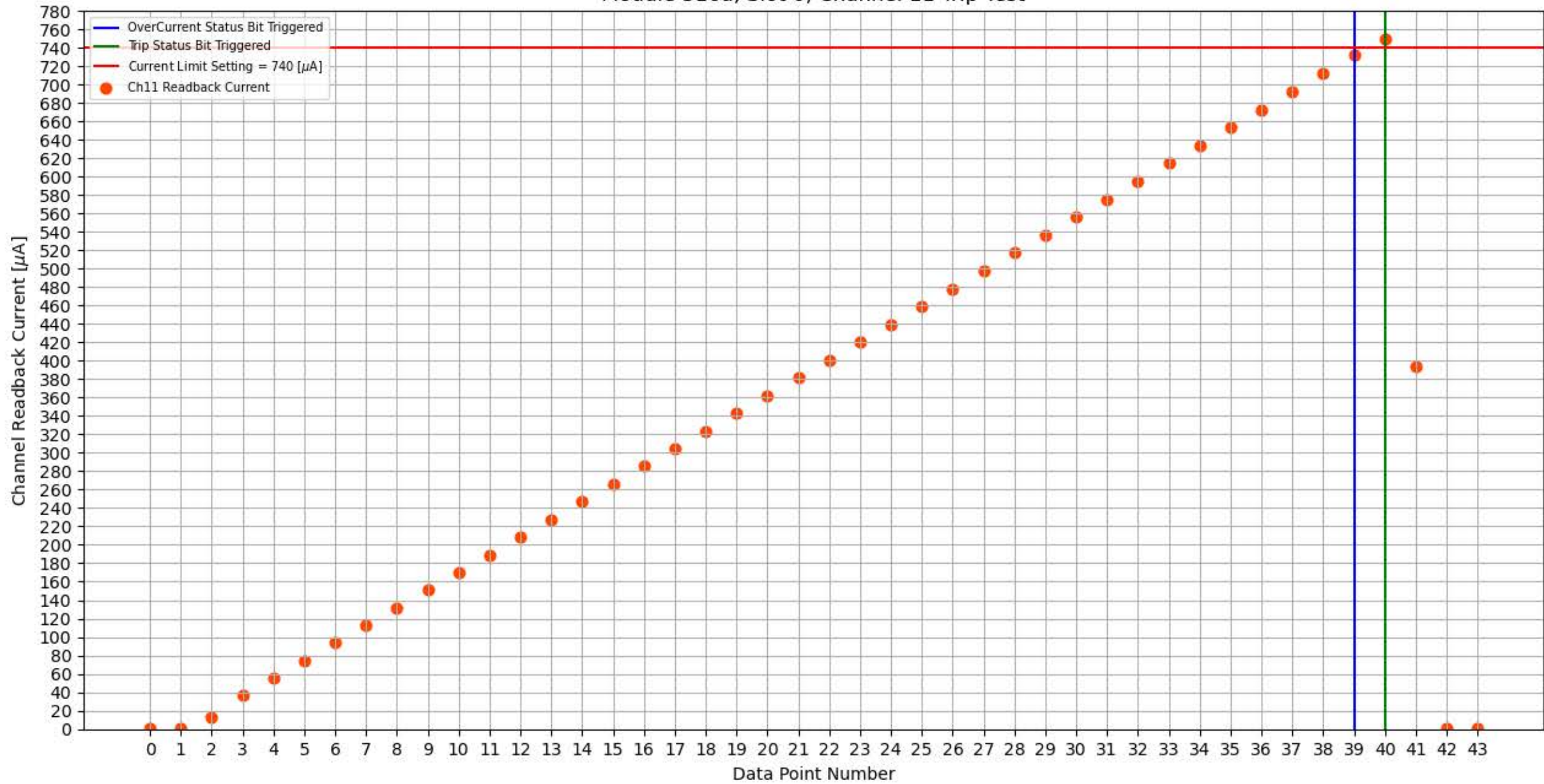
Module 316a, Slot 0, Channel 11 Trip Test
