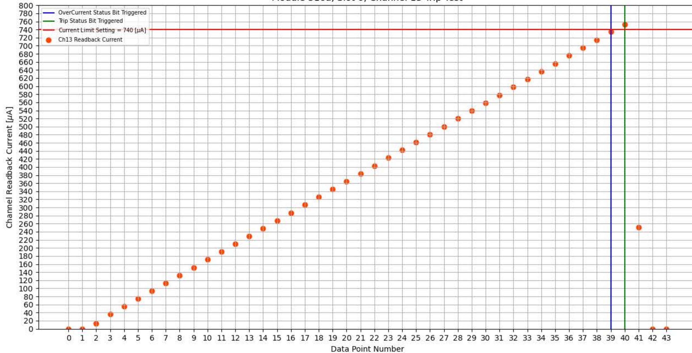
Module 316a, Slot 0, Channel 13 Trip Test
