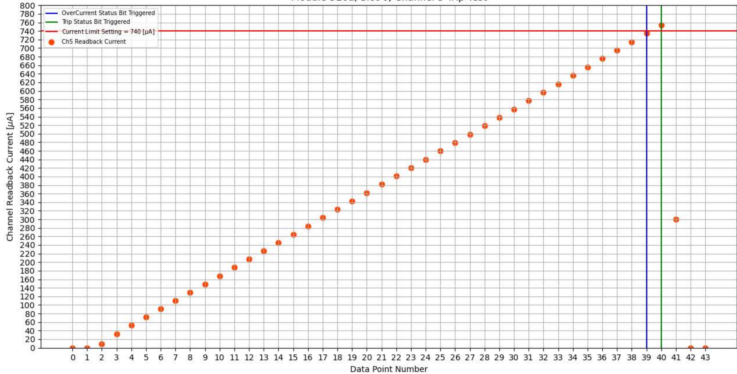
Module 316a, Slot 0, Channel 5 Trip Test
