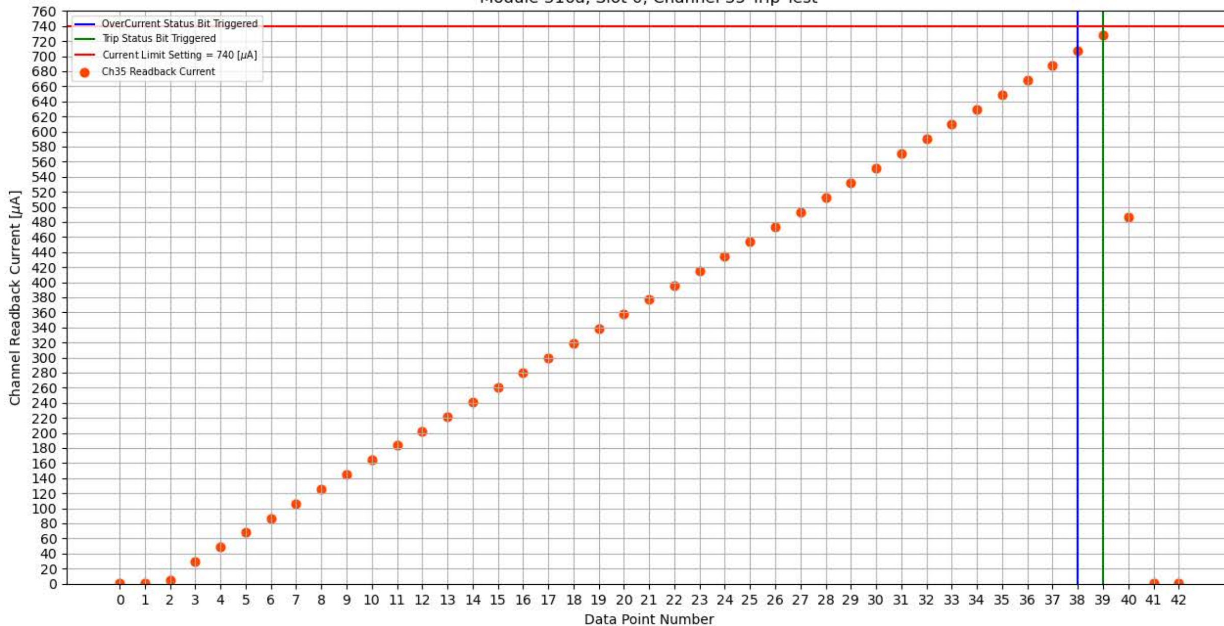
Module 316a, Slot 0, Channel 35 Trip Test
