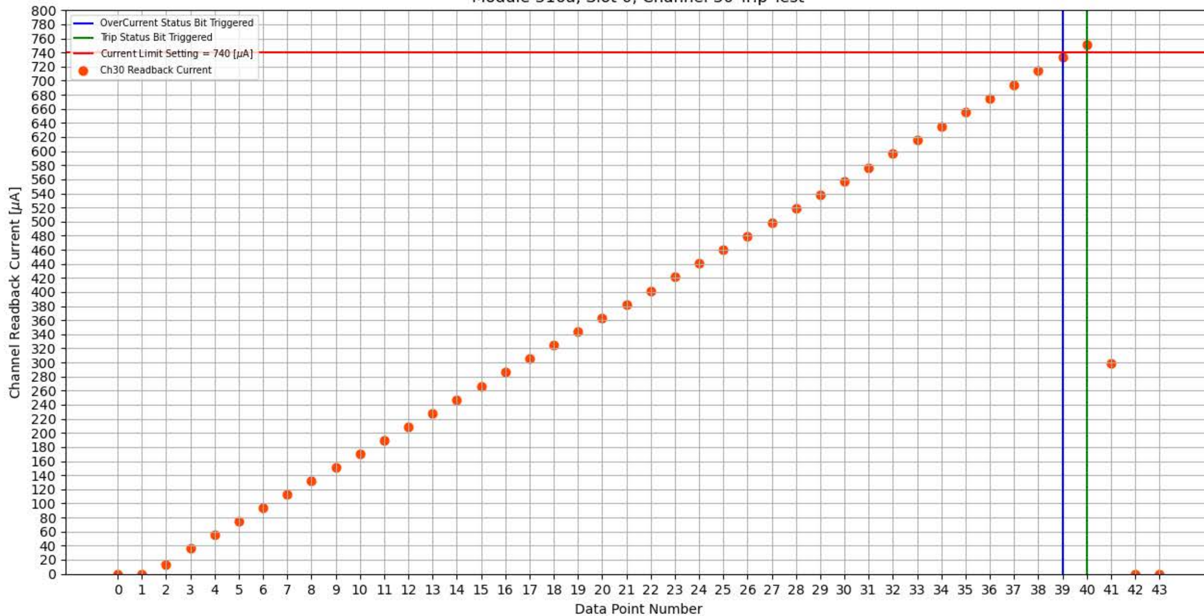
Module 316a, Slot 0, Channel 30 Trip Test
