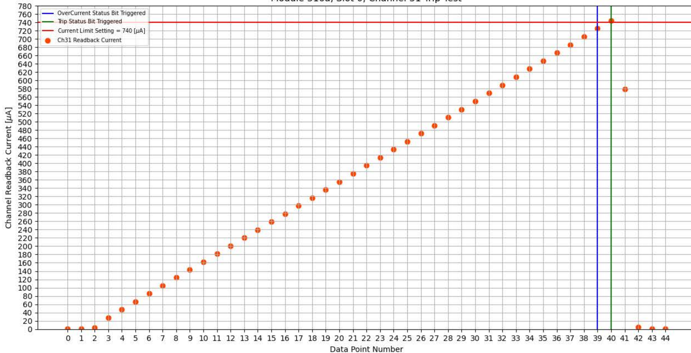
Module 316a, Slot 0, Channel 31 Trip Test
