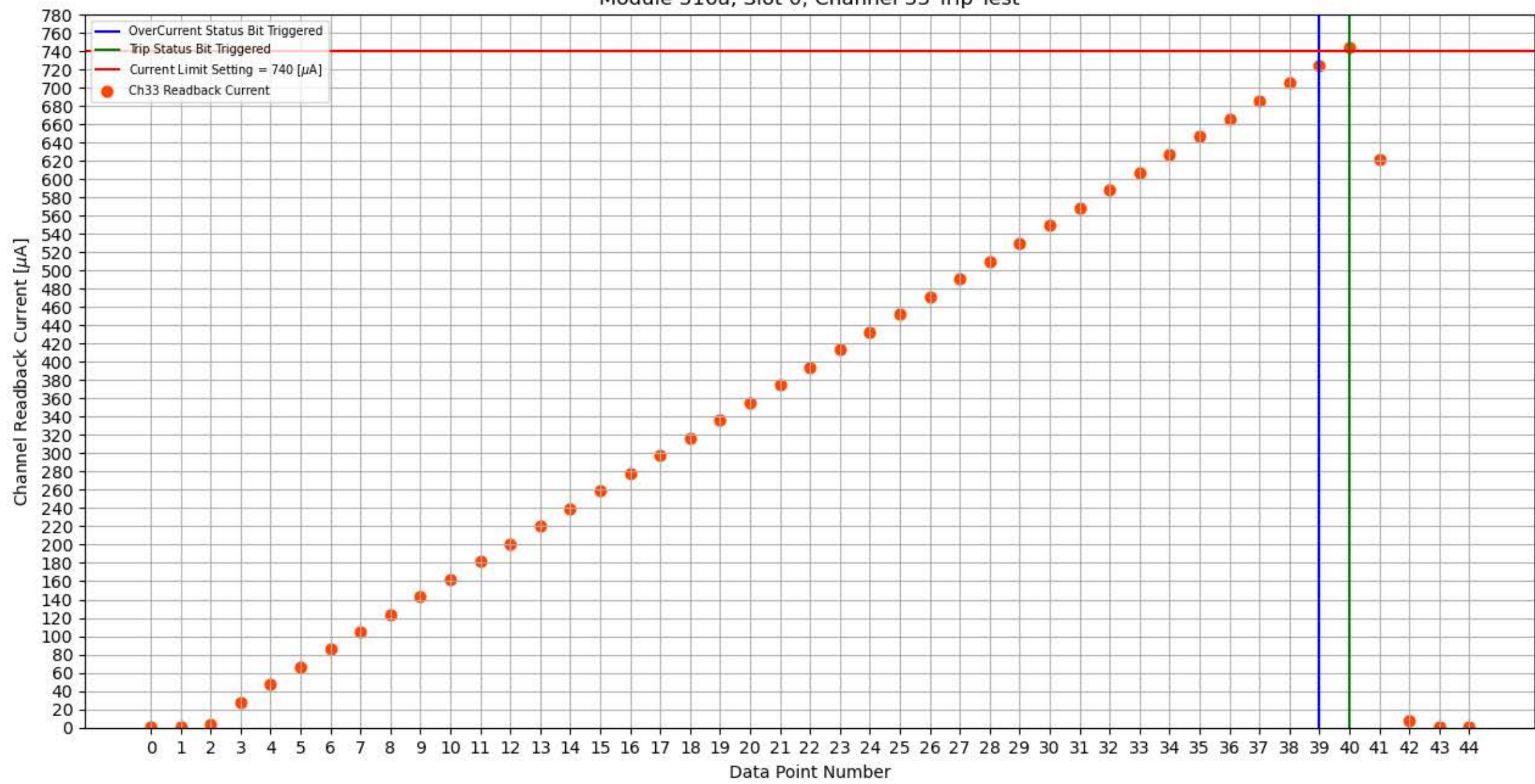
Module 316a, Slot 0, Channel 33 Trip Test
