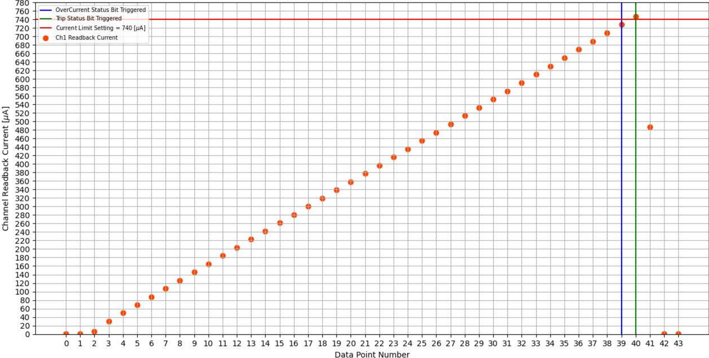
Module 316a, Slot 0, Channel 1 Trip Test
