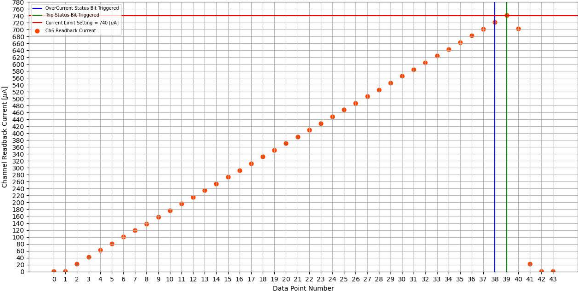
Module 316a, Slot 0, Channel 6 Trip Test
