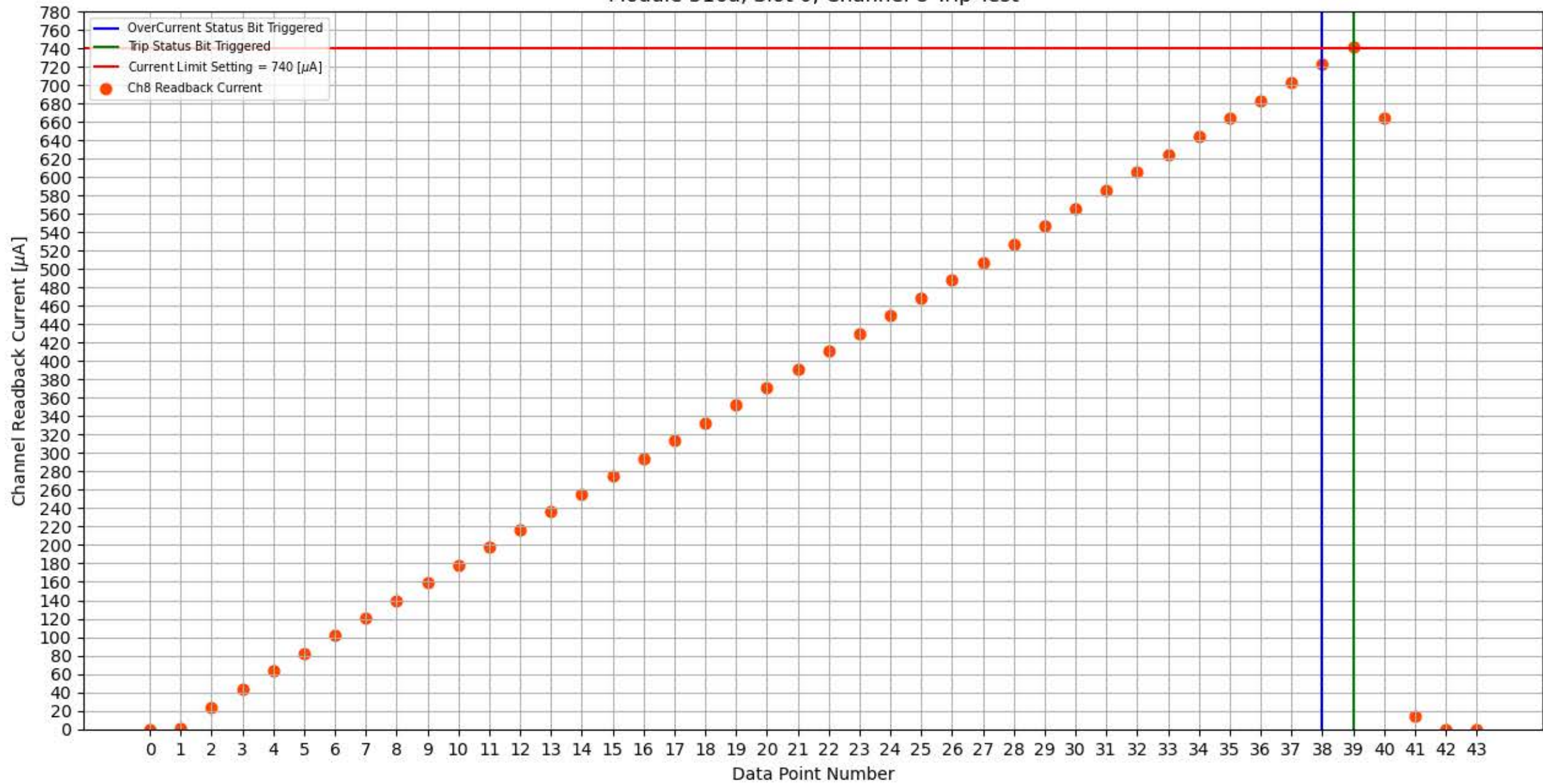
Module 316a, Slot 0, Channel 8 Trip Test
