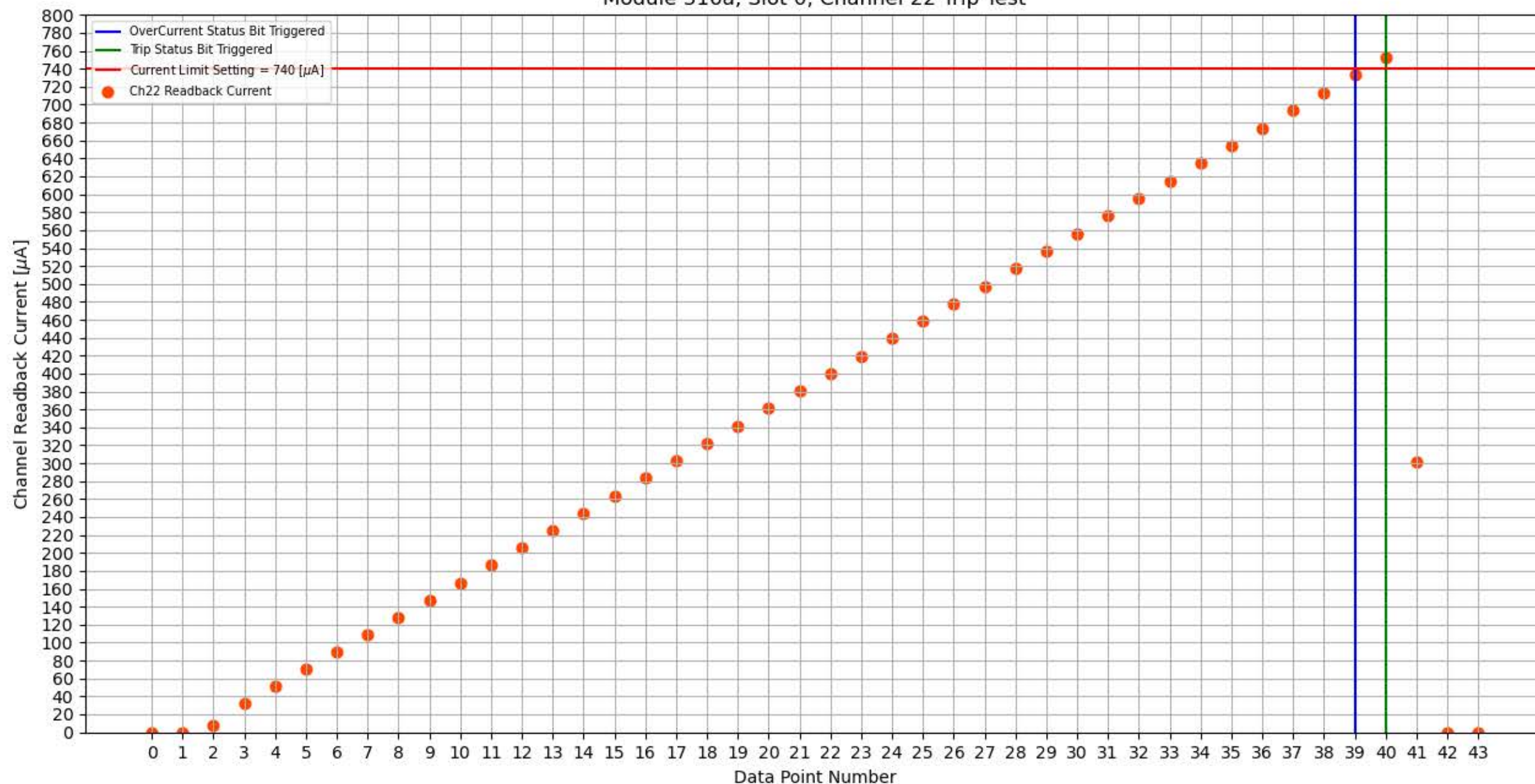
Module 316a, Slot 0, Channel 22 Trip Test
