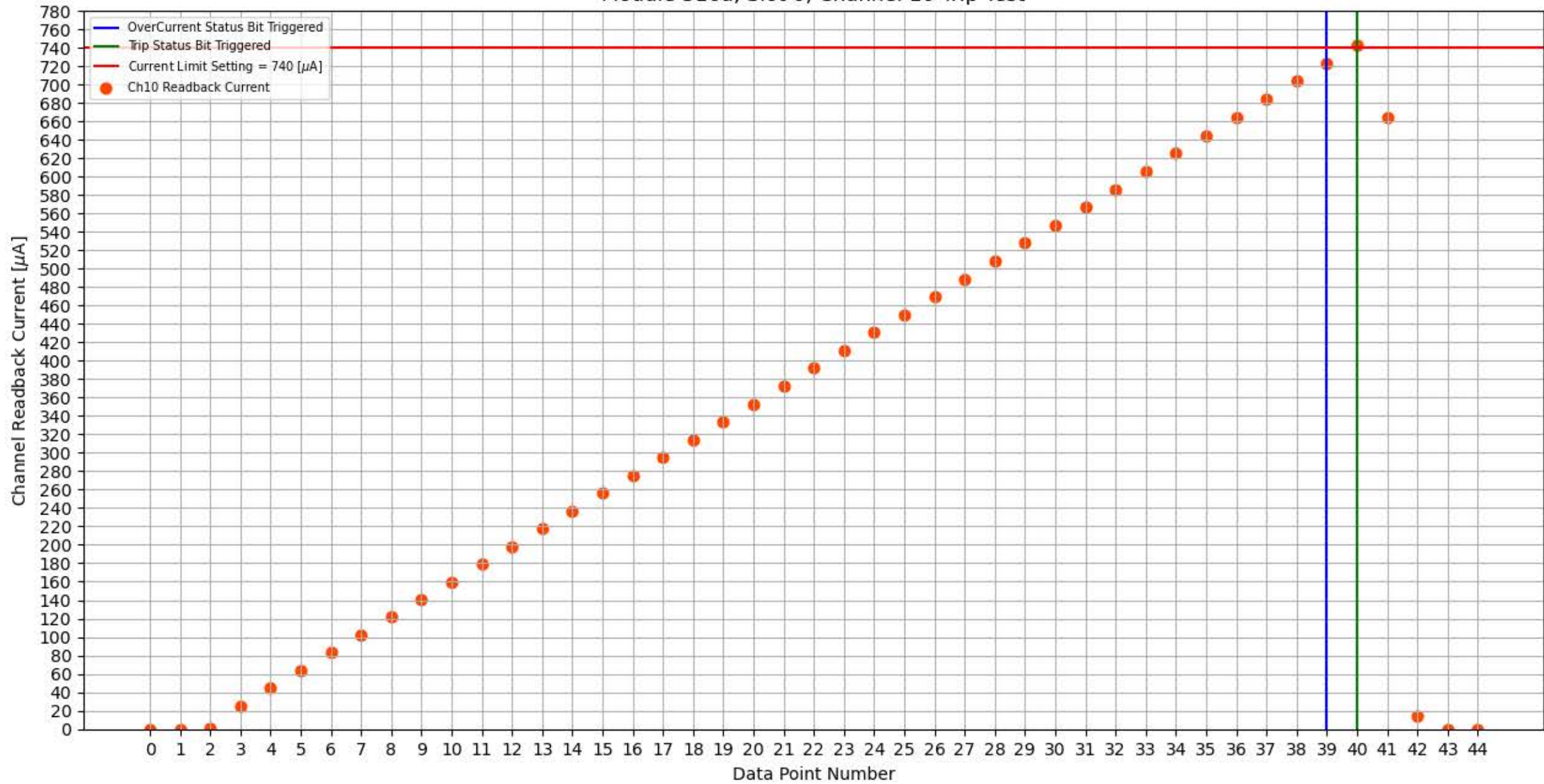
Module 316a, Slot 0, Channel 10 Trip Test
