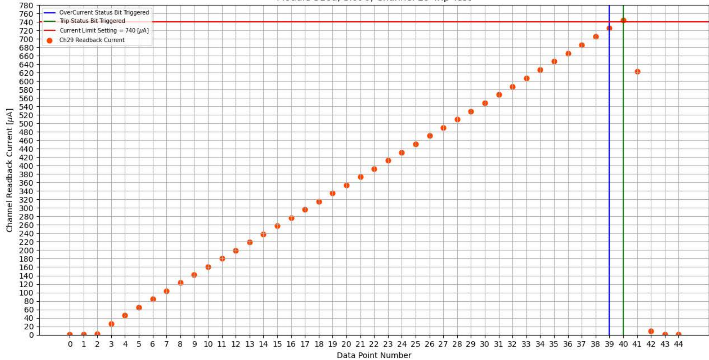
Module 316a, Slot 0, Channel 29 Trip Test
