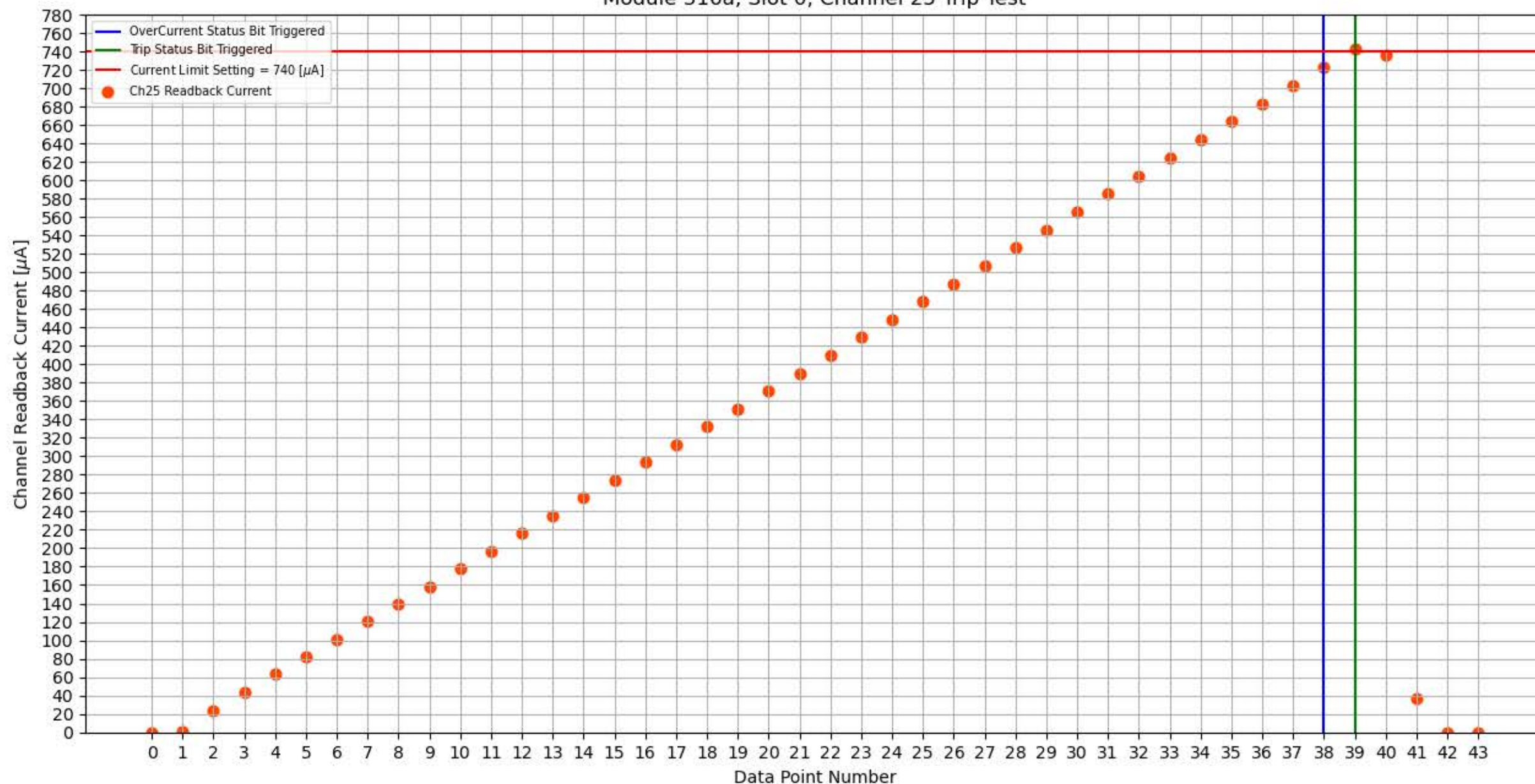
Module 316a, Slot 0, Channel 25 Trip Test
