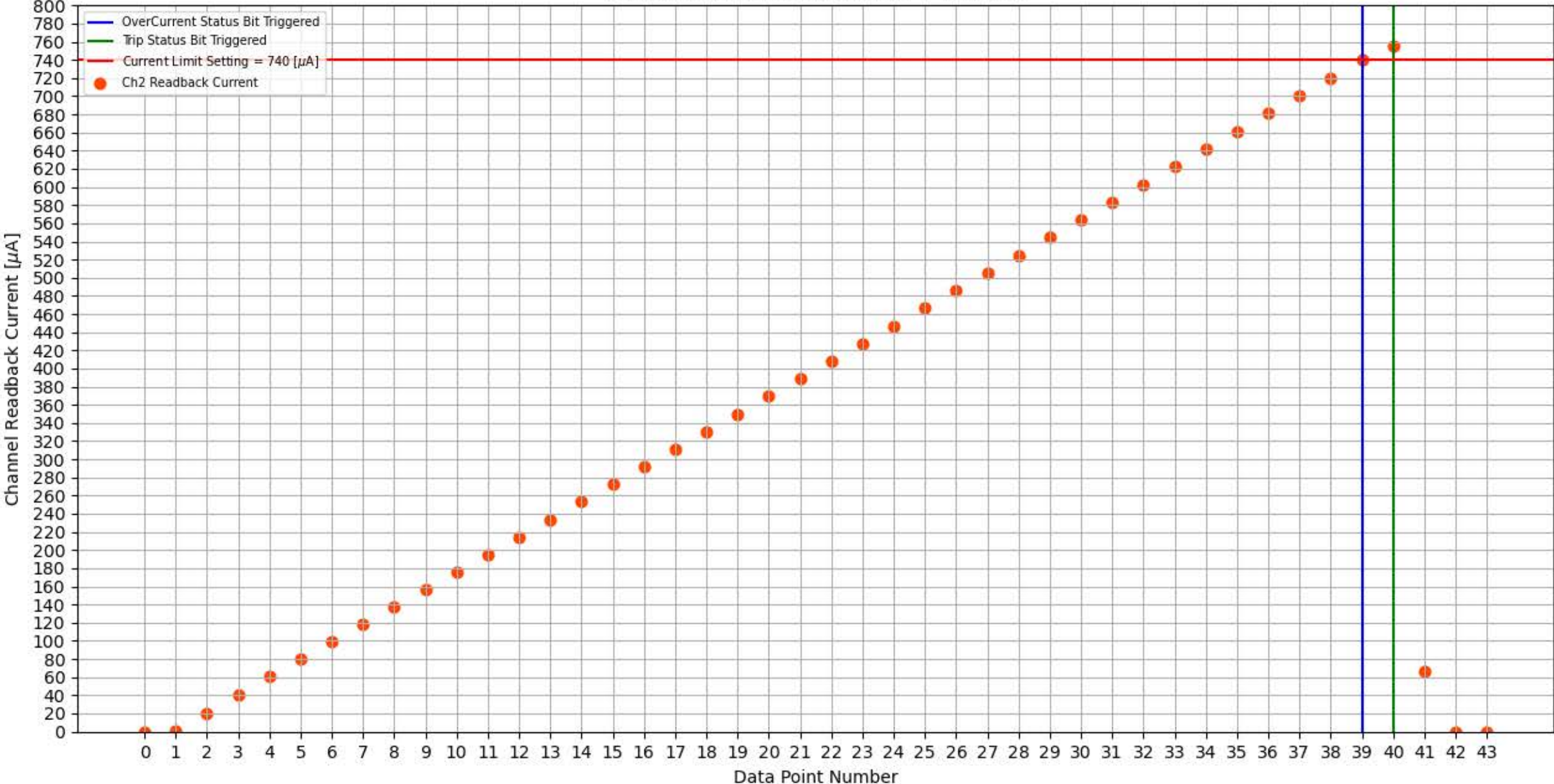
Module 316a, Slot 0, Channel 2 Trip Test
