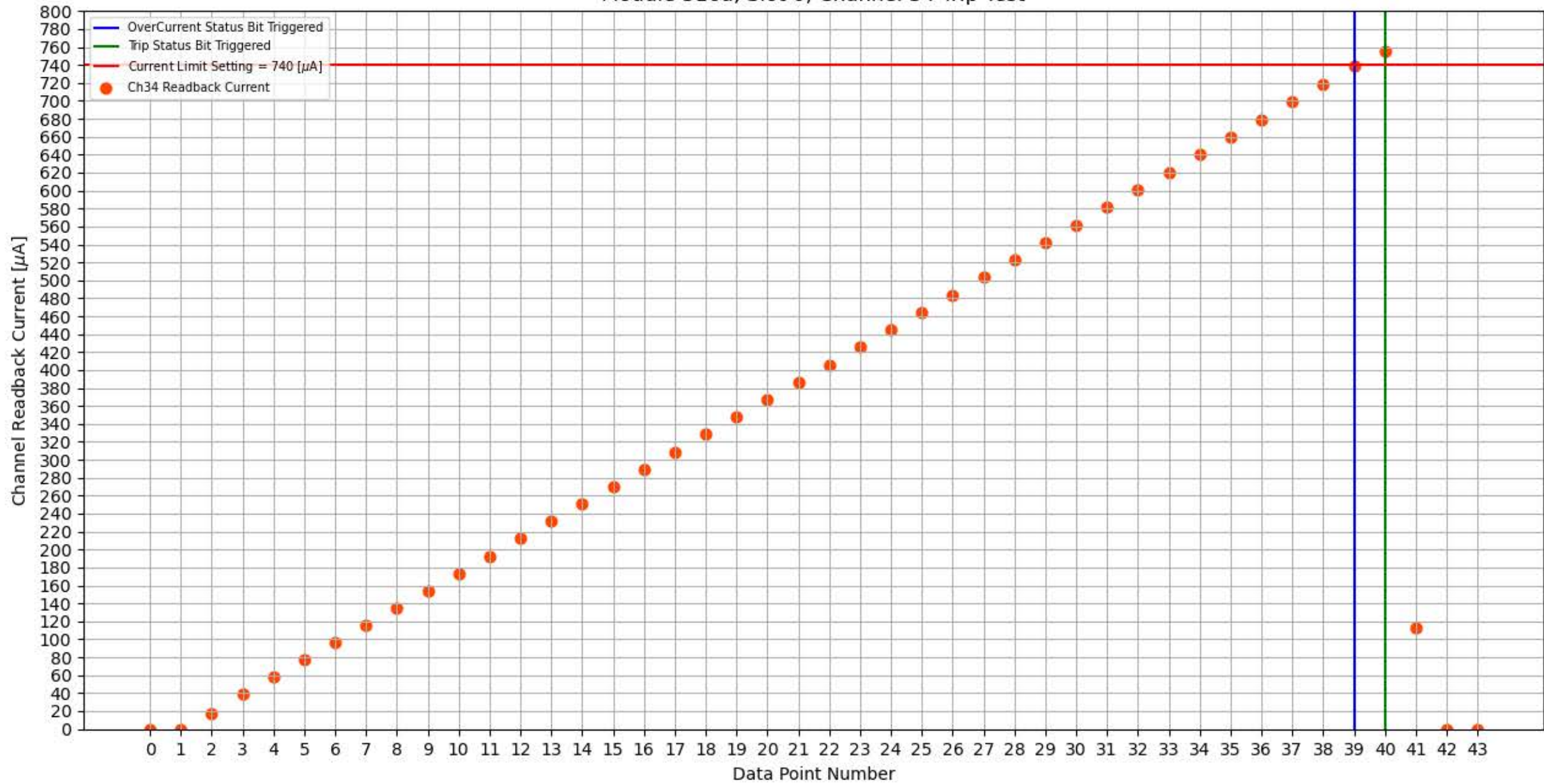
Module 316a, Slot 0, Channel 34 Trip Test
