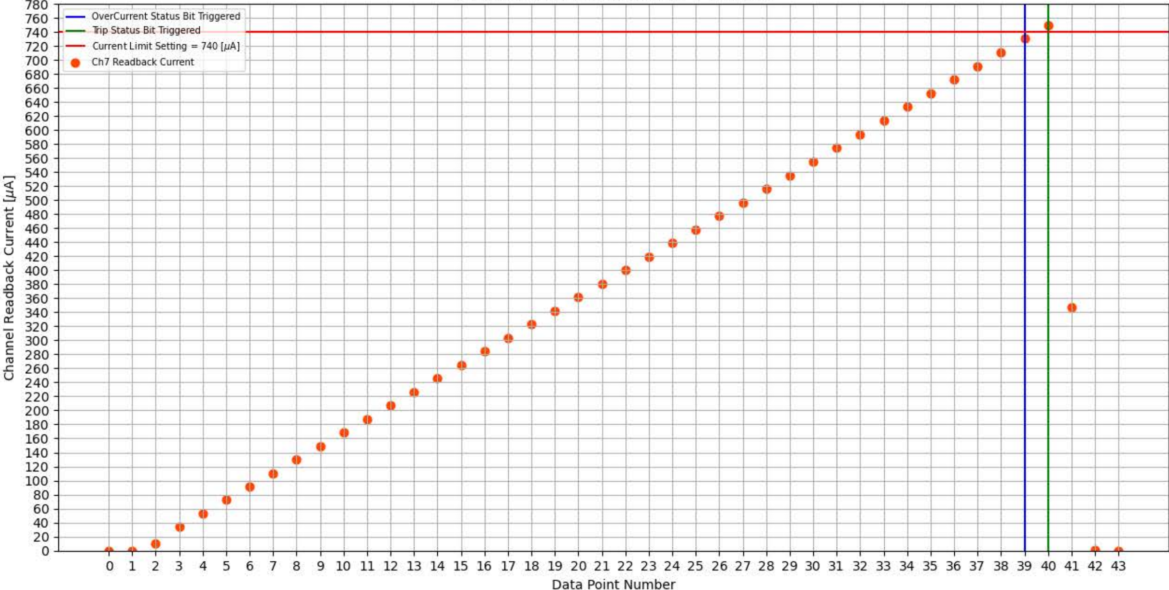
Module 316a, Slot 0, Channel 7 Trip Test
