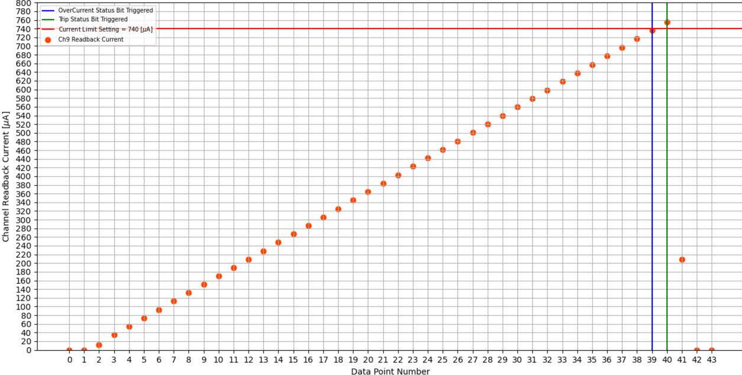
Module 316a, Slot 0, Channel 9 Trip Test
