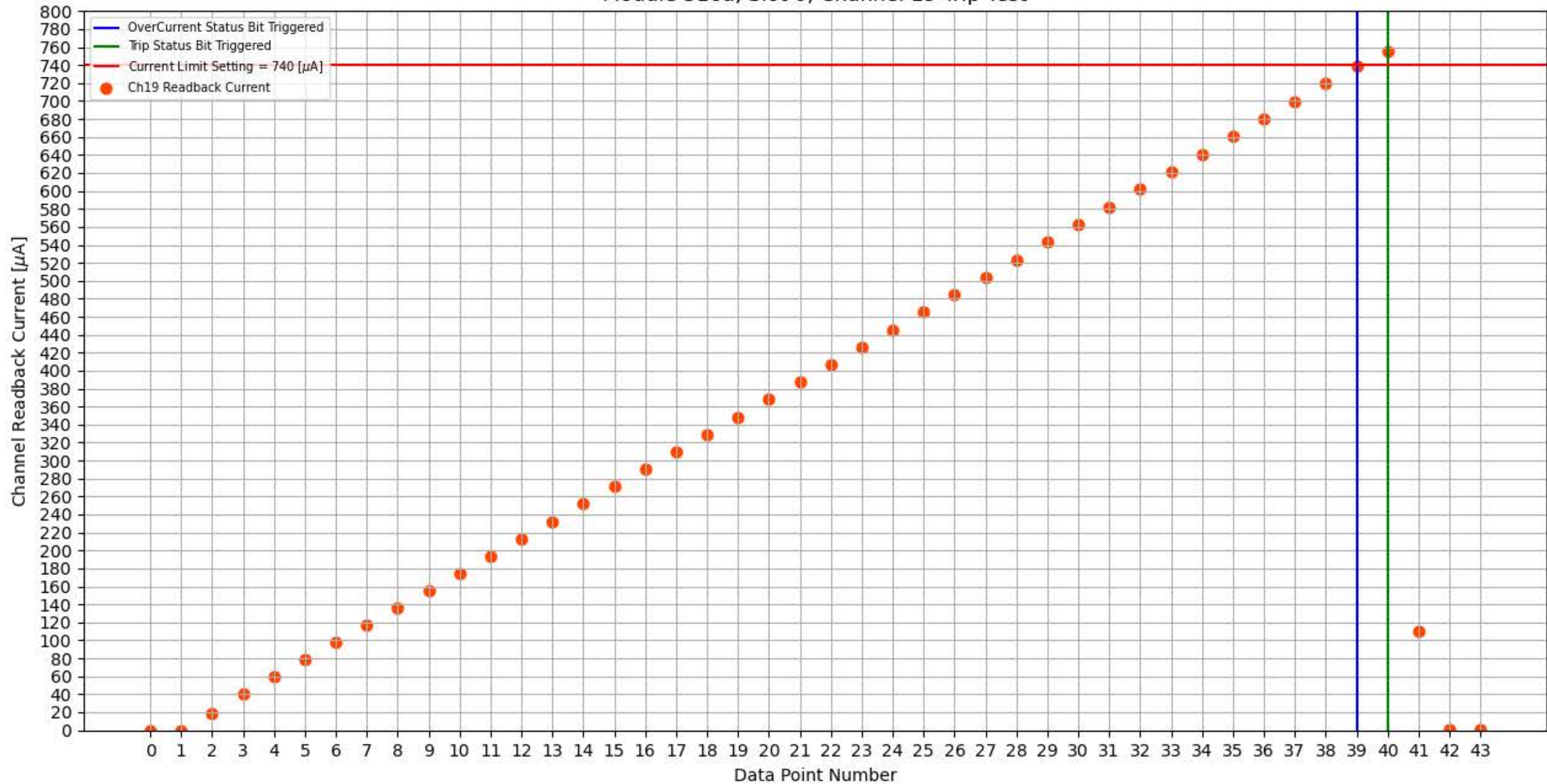
Module 316a, Slot 0, Channel 19 Trip Test
