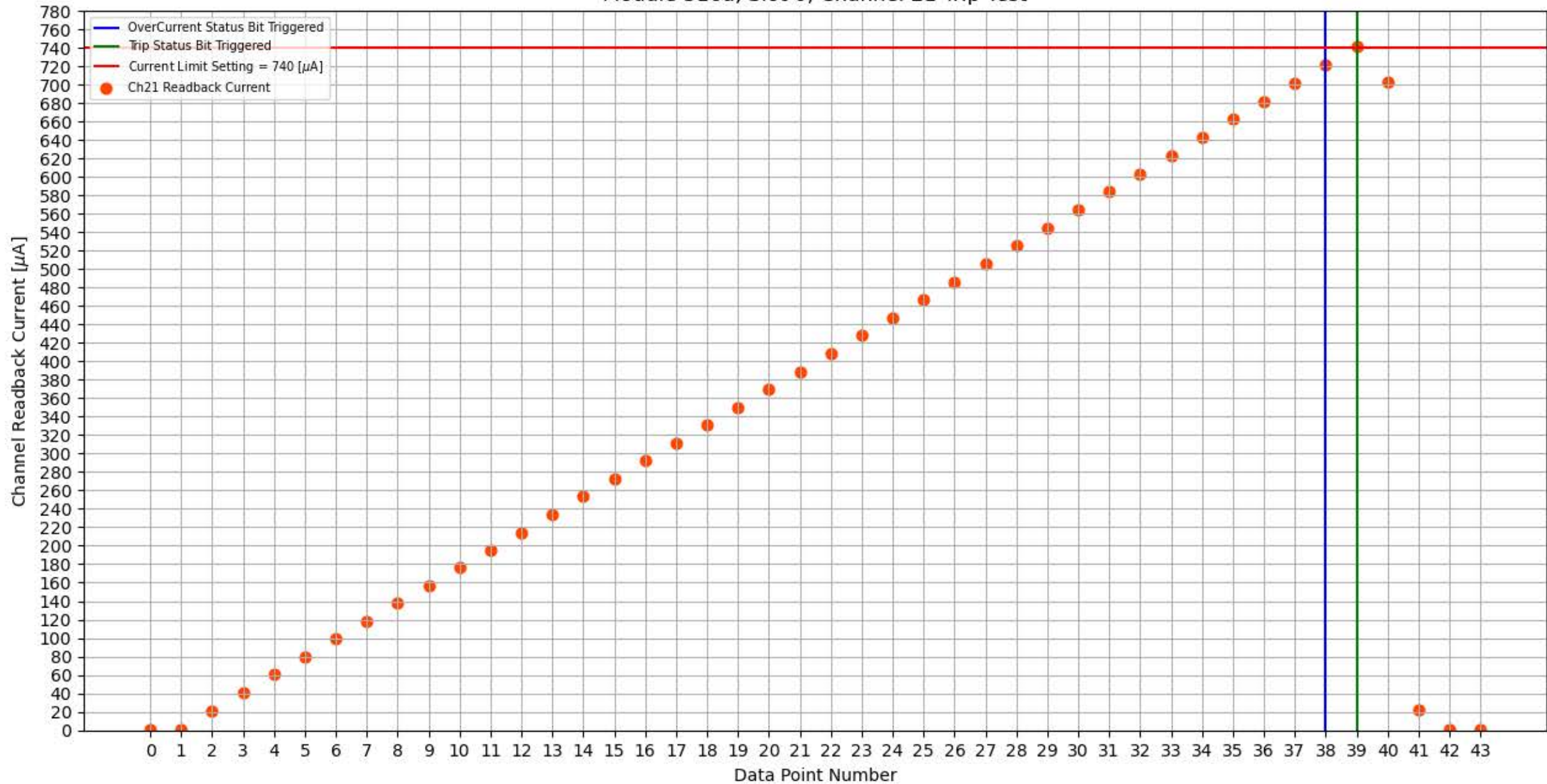
Module 316a, Slot 0, Channel 21 Trip Test
