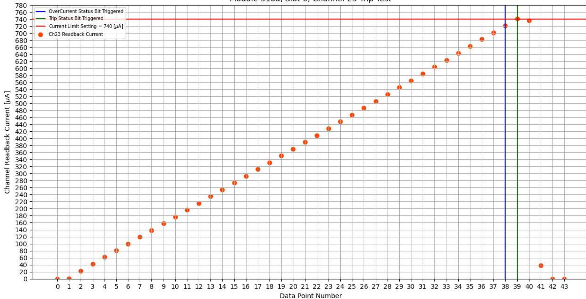
Module 316a, Slot 0, Channel 23 Trip Test
