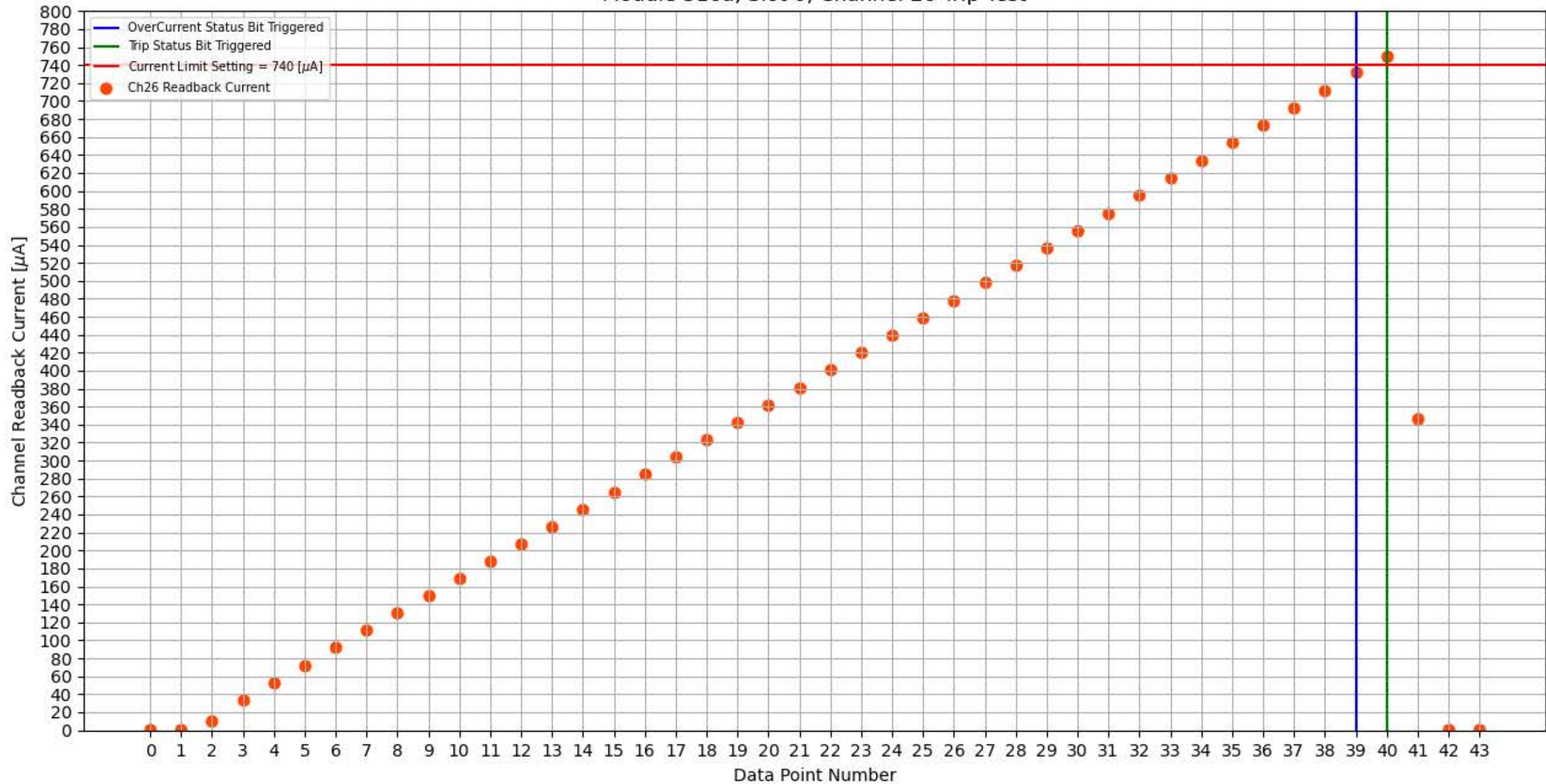
Module 316a, Slot 0, Channel 26 Trip Test
