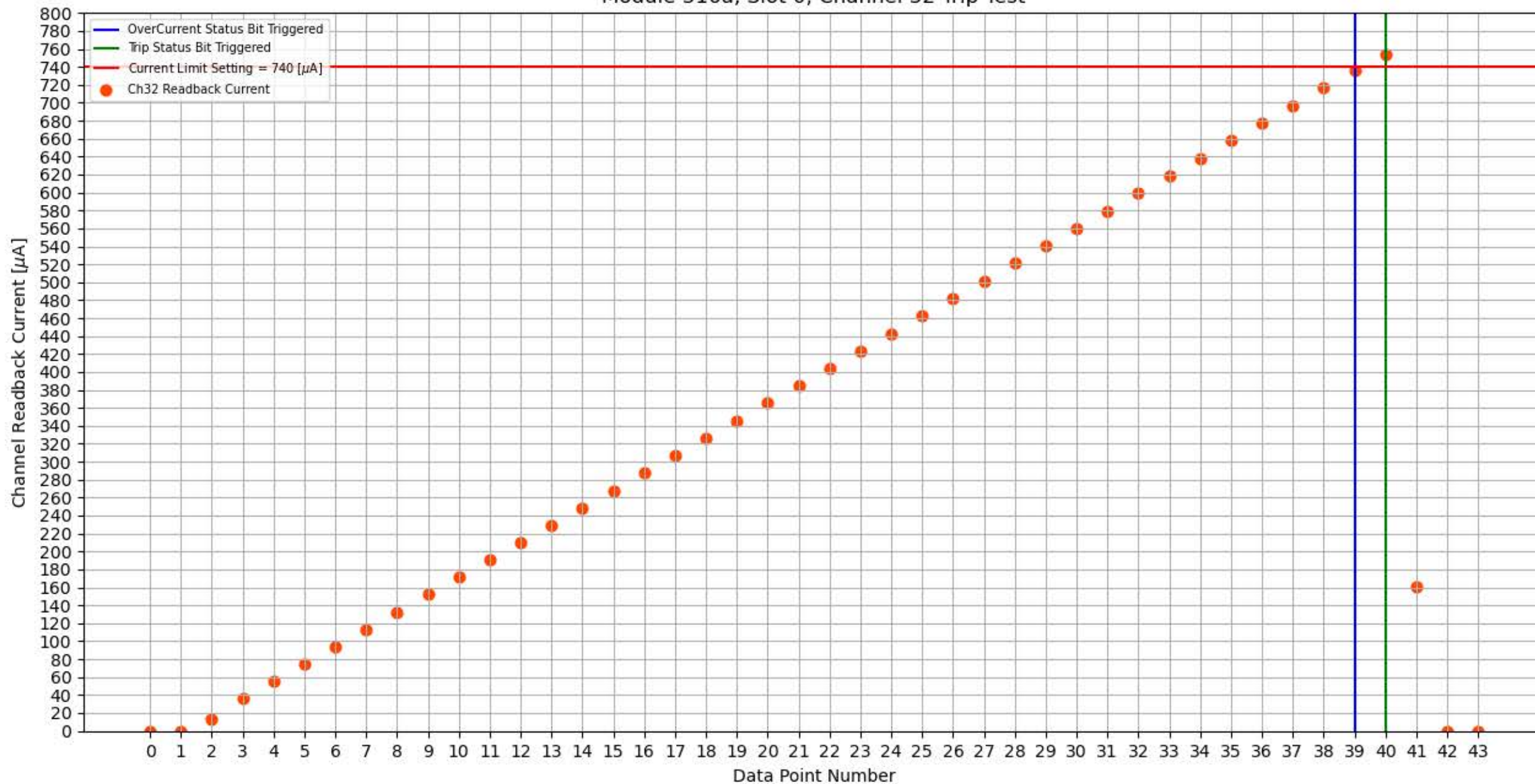
Module 316a, Slot 0, Channel 32 Trip Test
