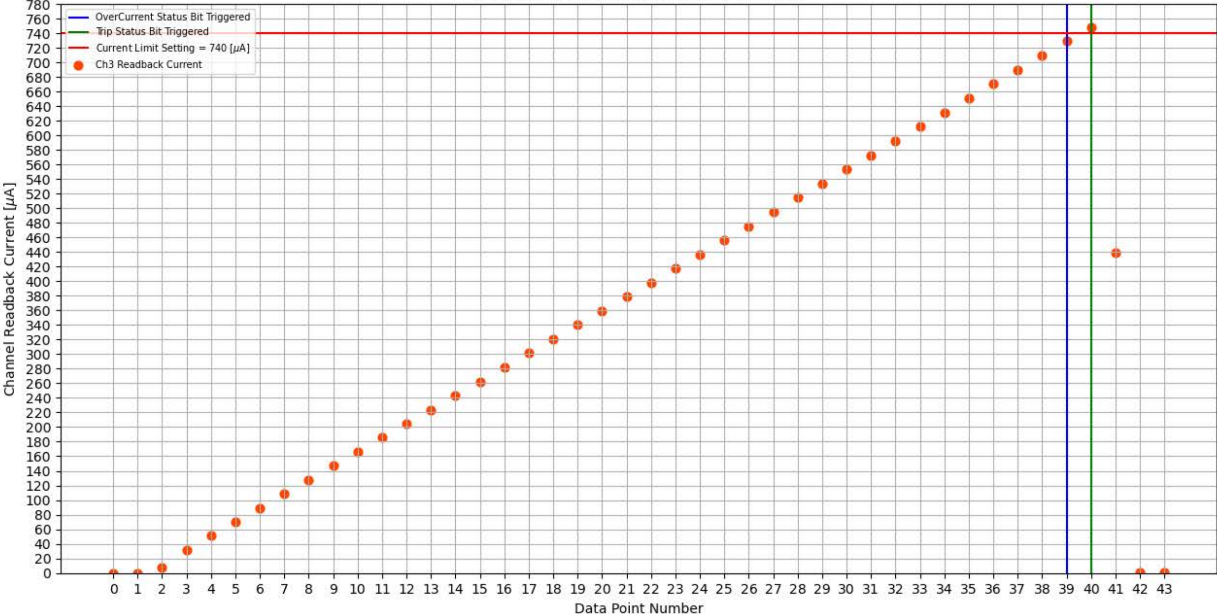
Module 316a, Slot 0, Channel 3 Trip Test
