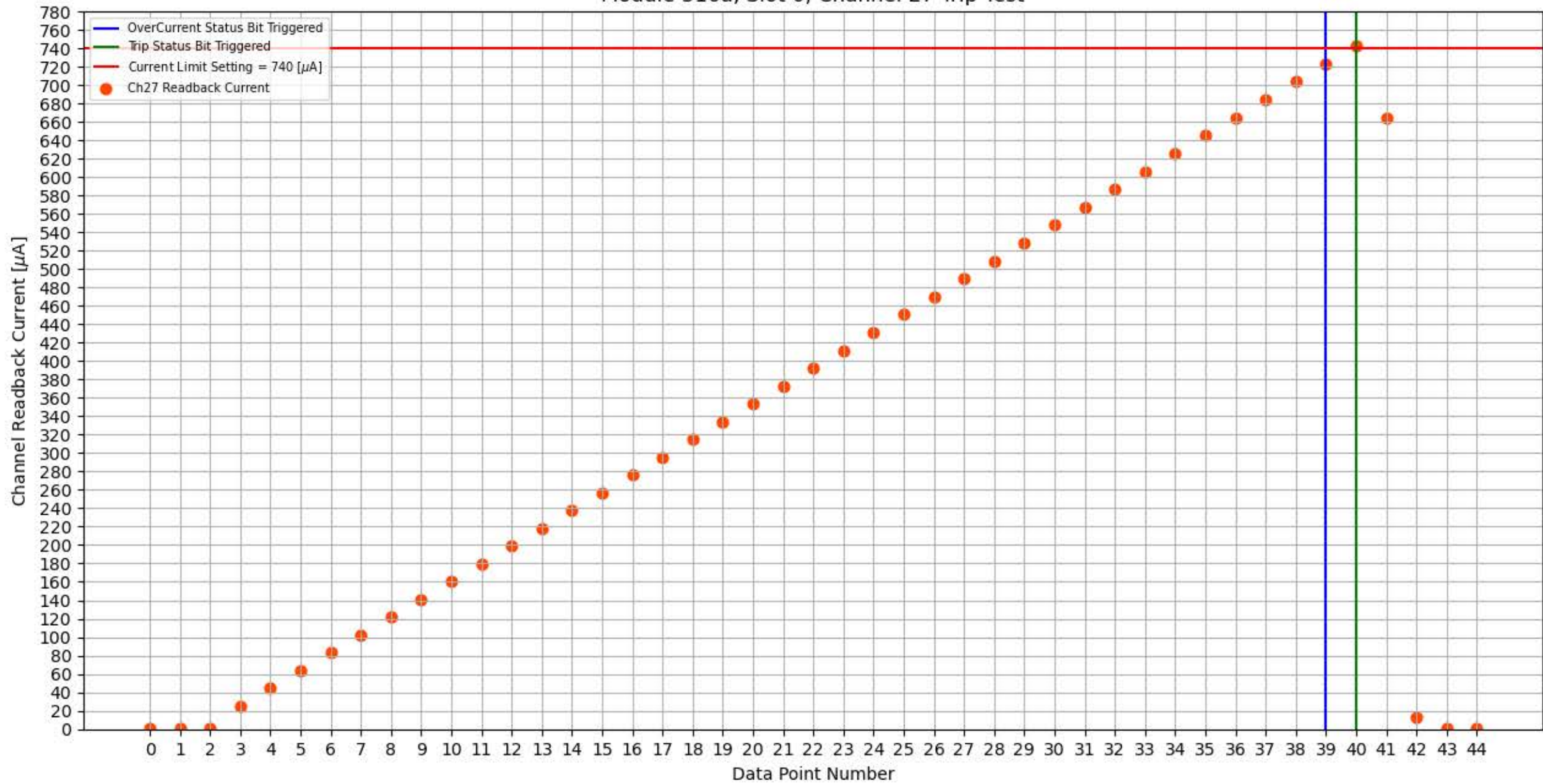
Module 316a, Slot 0, Channel 27 Trip Test
