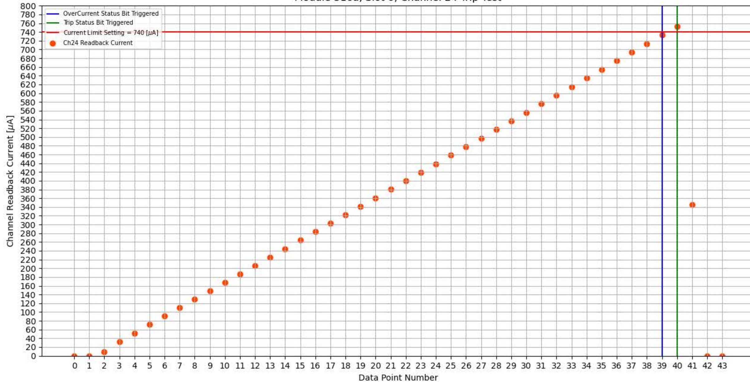
Module 316a, Slot 0, Channel 24 Trip Test
