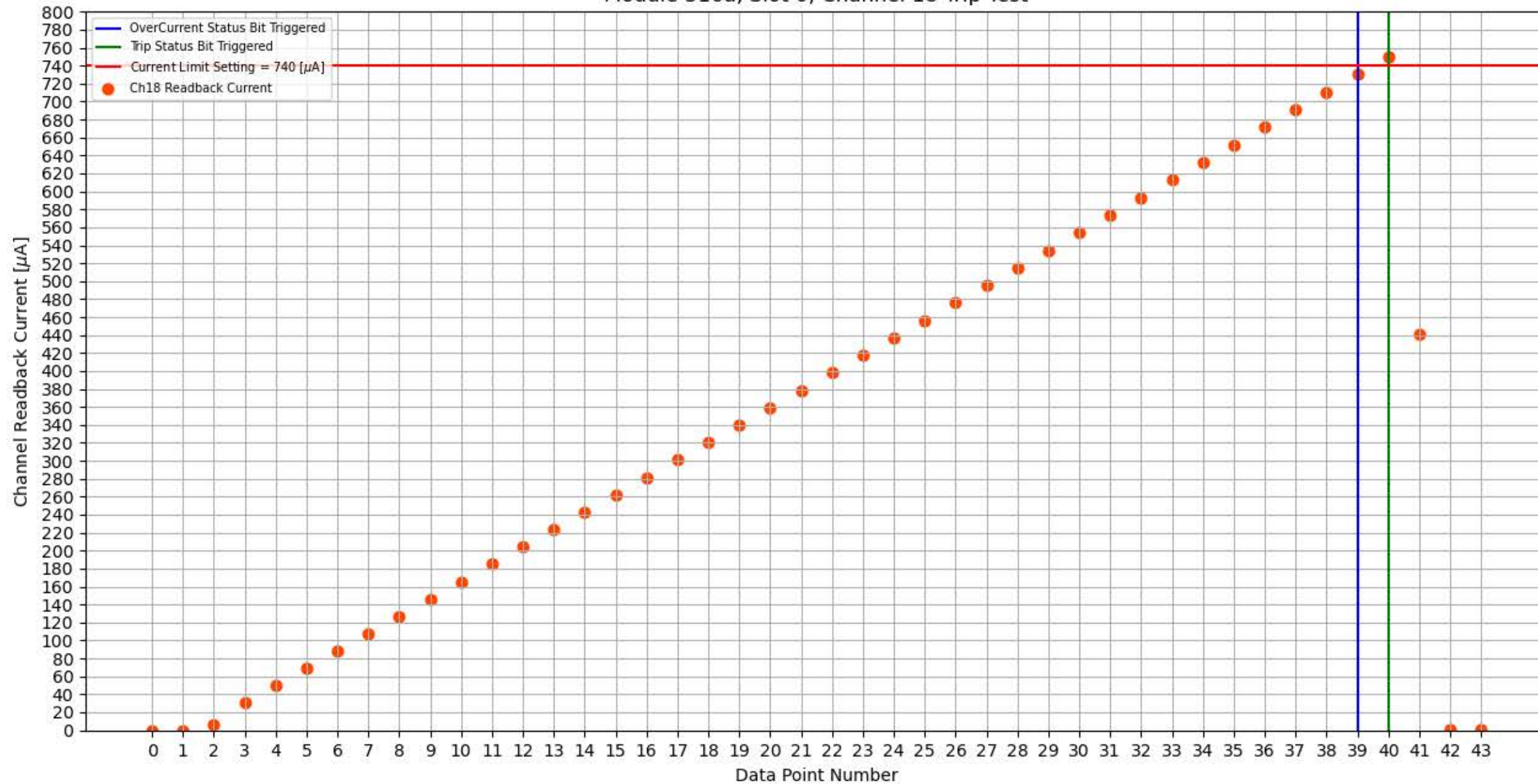
Module 316a, Slot 0, Channel 18 Trip Test
