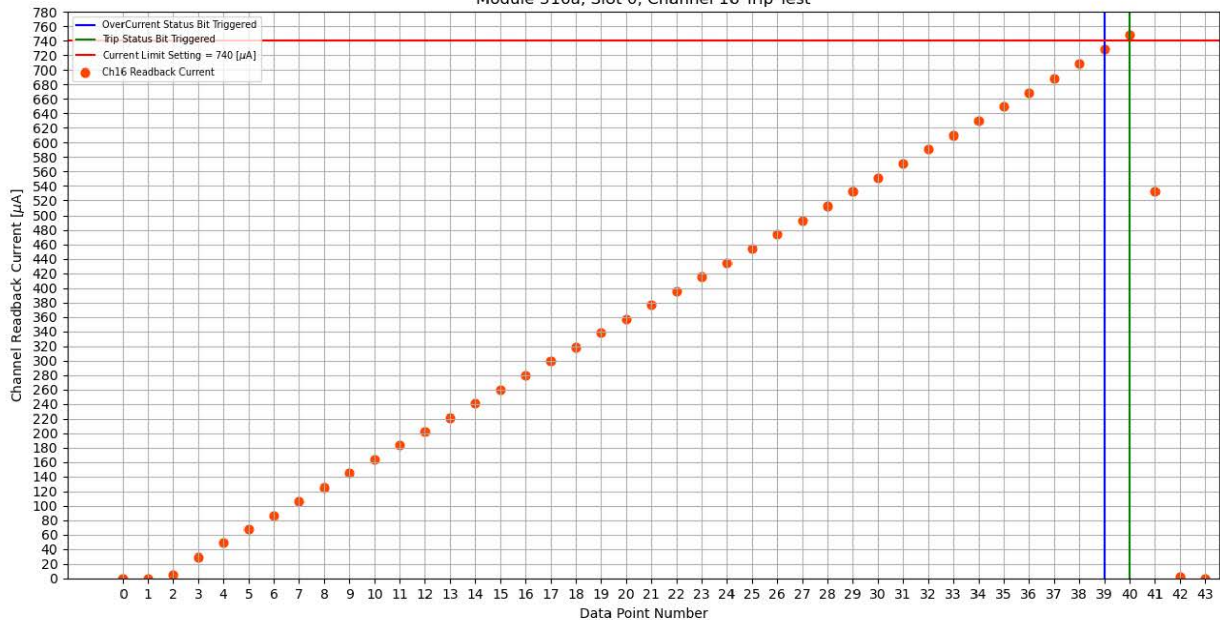
Module 316a, Slot 0, Channel 16 Trip Test
