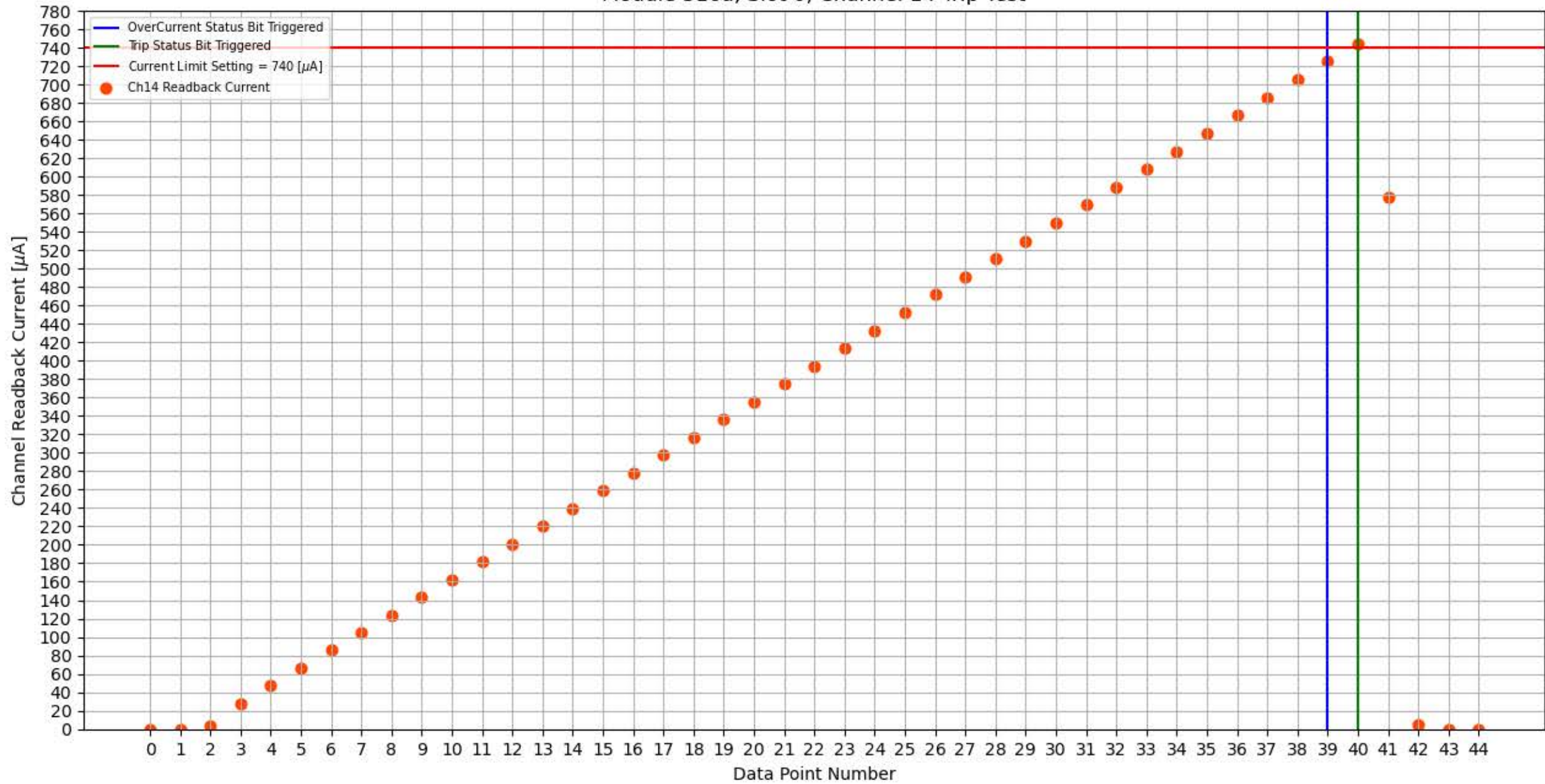
Module 316a, Slot 0, Channel 14 Trip Test
