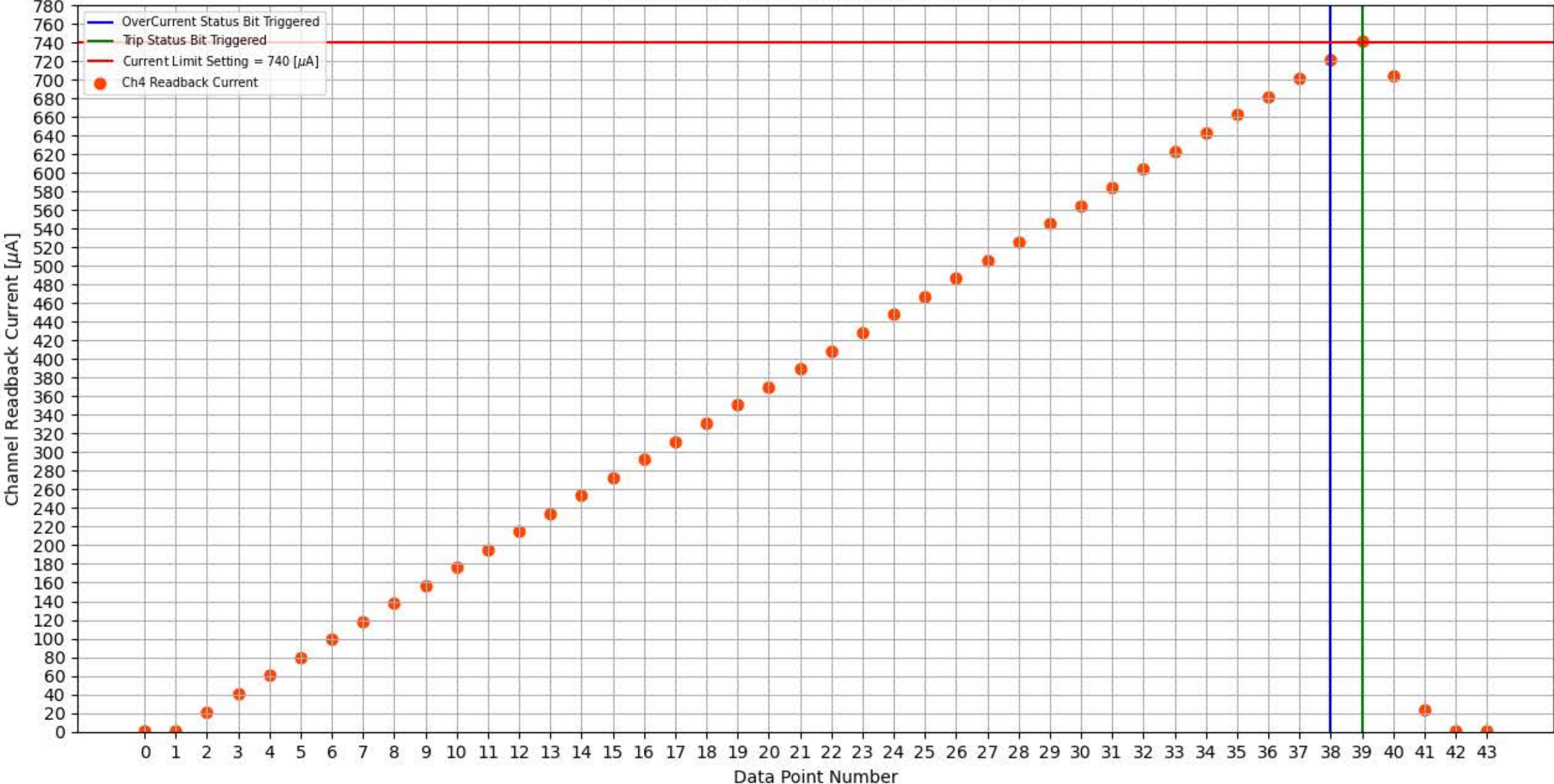
Module 316a, Slot 0, Channel 4 Trip Test
