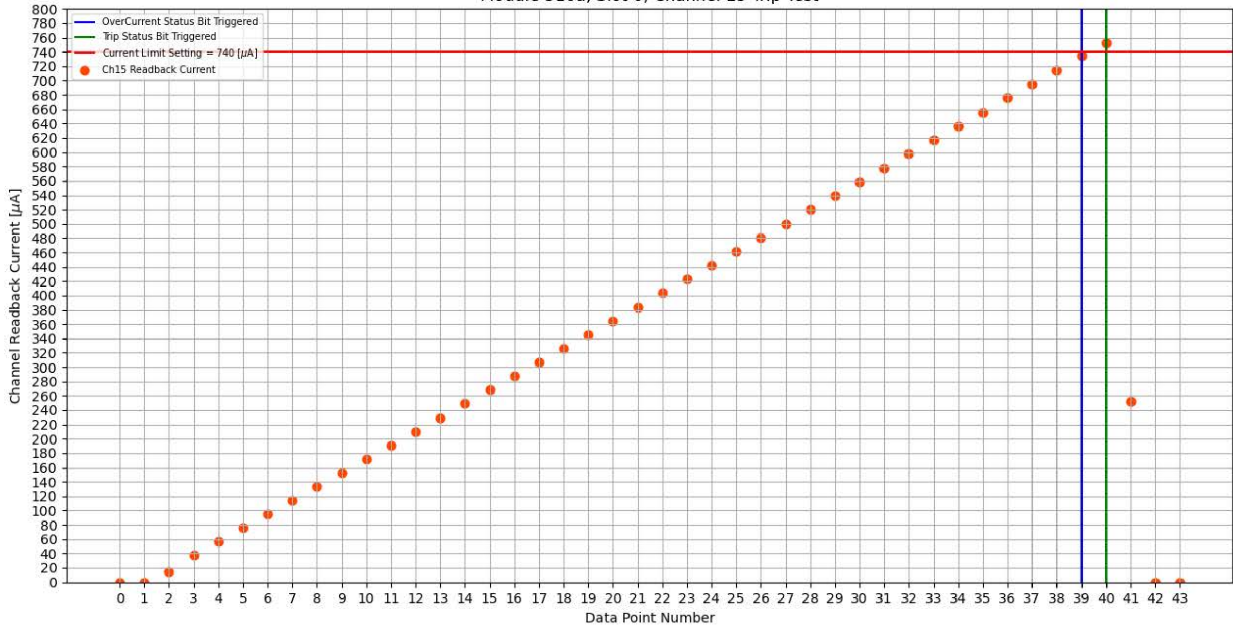
Module 316a, Slot 0, Channel 15 Trip Test
