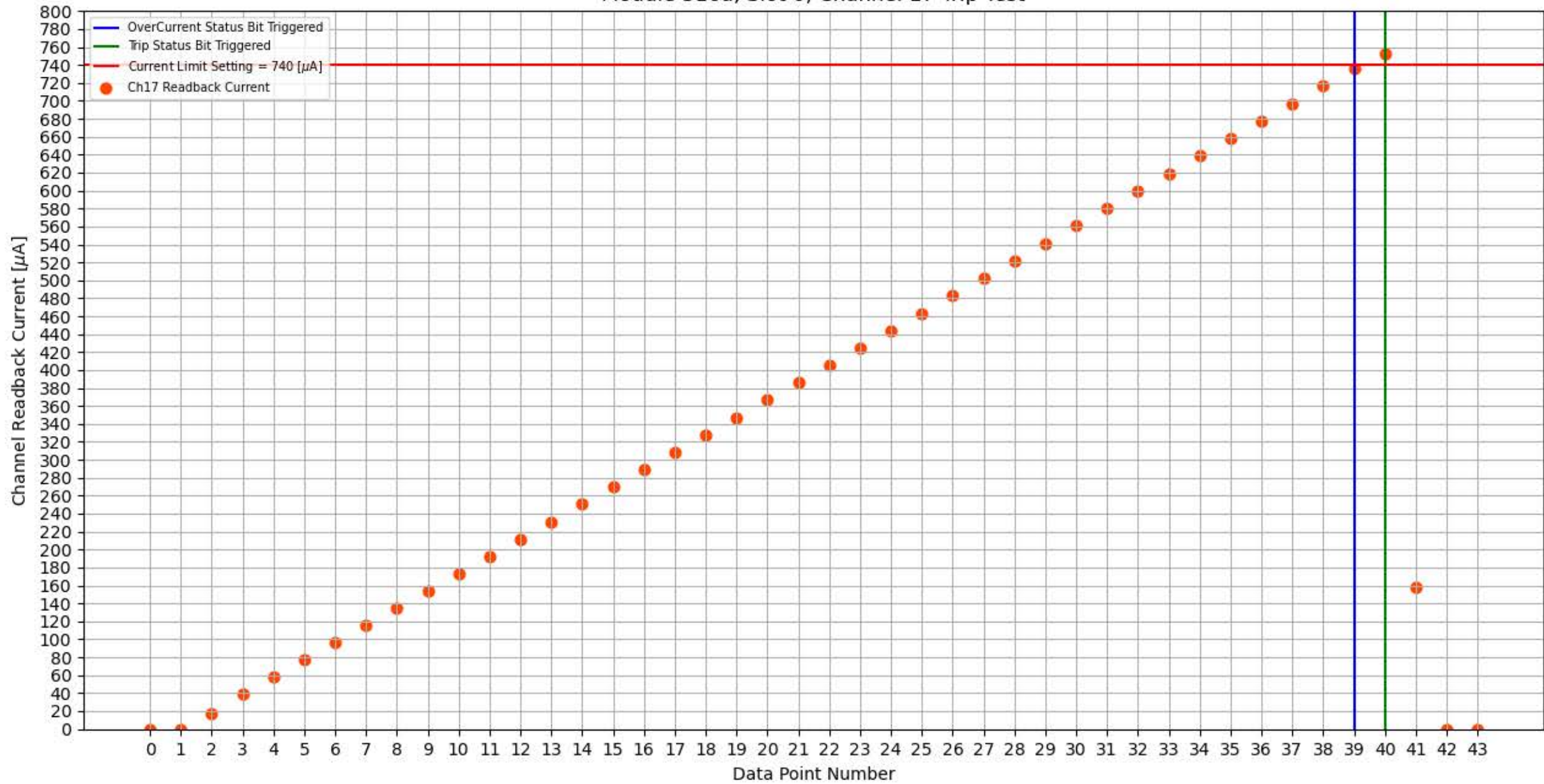
Module 316a, Slot 0, Channel 17 Trip Test
